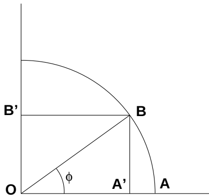
FIGURE 2.5.1. Trigonometric integrals
