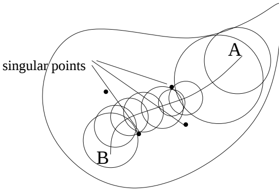
FIGURE 3.6.1. Analytic continuation
