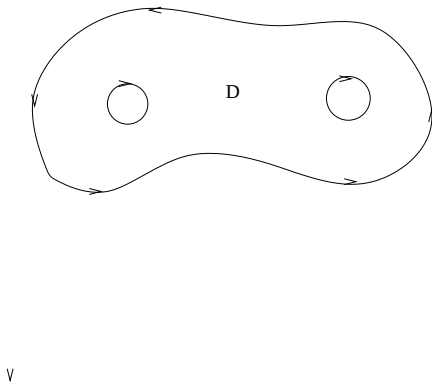
FIGURE 3.5.1. Contour integral
